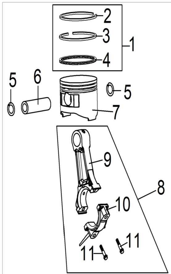
PISTON & BIELA
